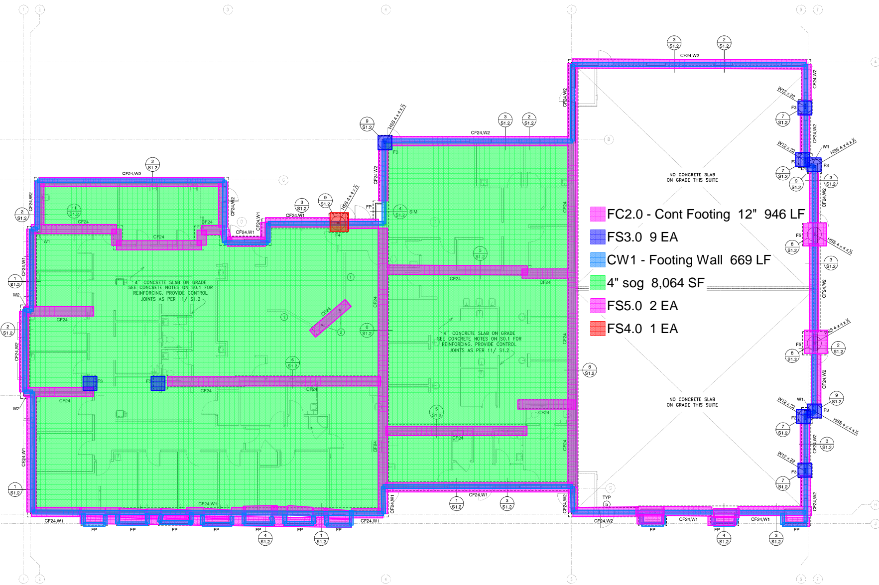
FOOTING SCHEDULE
